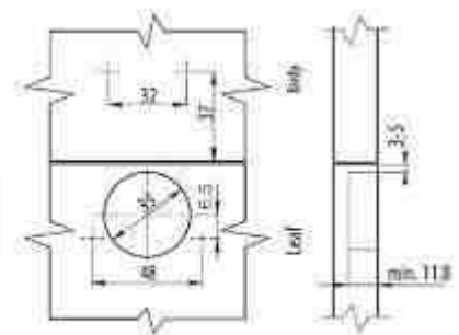
Mounting Dimensions
